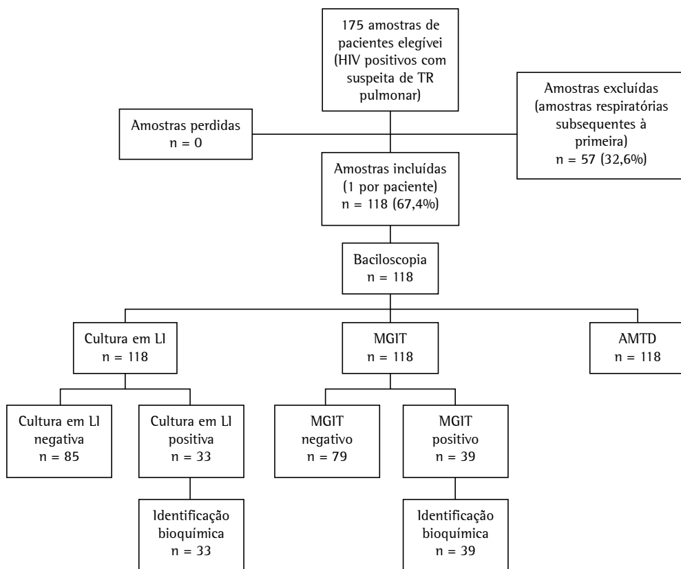
Figura 2 – Diagrama do estudo. TB: tuberculose; LJ: Löwenstein-Jensen; MGIT: Mycobacteria Growth Indicator Tube ; e AMTD: teste amplified Mycobacterium tuberculosis direct .
