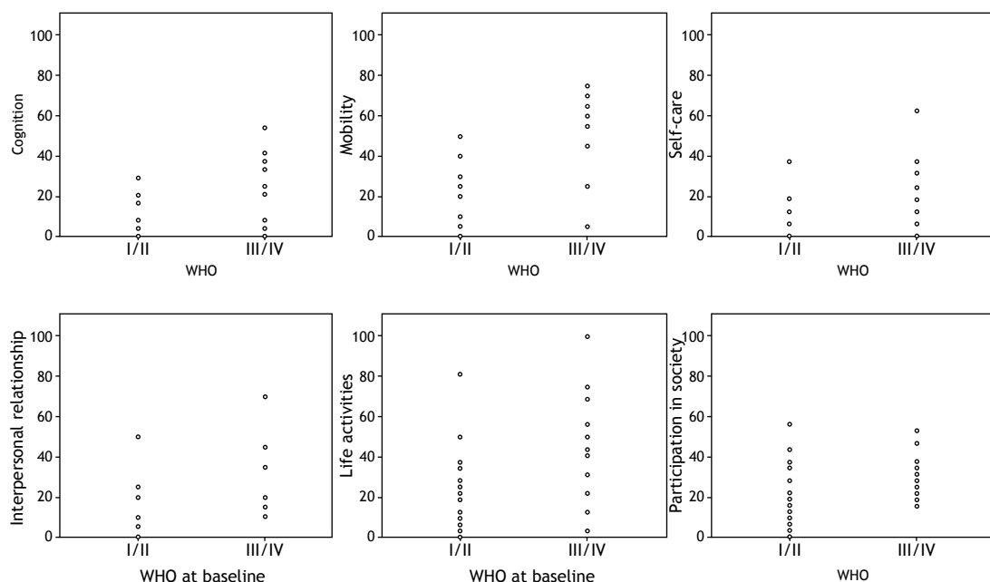
Figure S2. Scatterplots for correlations between World Health Organization Disability Assessment Schedule 2.0 (WHODAS 2.0) scores and World Health Organization (WHO) Functional Class.
